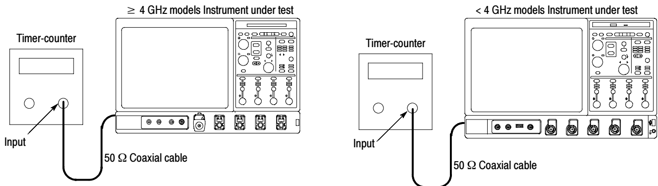
Figure 2-18: Initial test hookup
